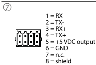
Serial interface, RS422 mode
