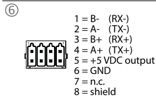
Serial interface, RS485 mode
