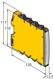
IMX12-DO01-2U-2U-0/24VDC
