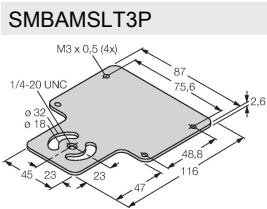
SMBAMSLT3P 3073132 Backplane, stainless steel, for LT3 series
